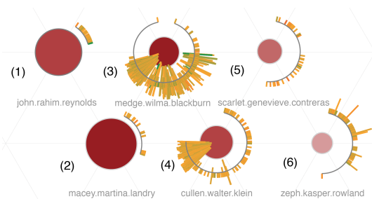
Fig. 11. Some anomalous users in the Enron Email data.
