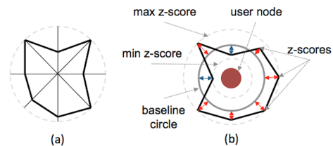
Fig. 6. Feature glyph design. (a) star-glyph; (b) z-glyph showing the differences in the feature values compared to the baseline circle which indicates the mean values of the features.
