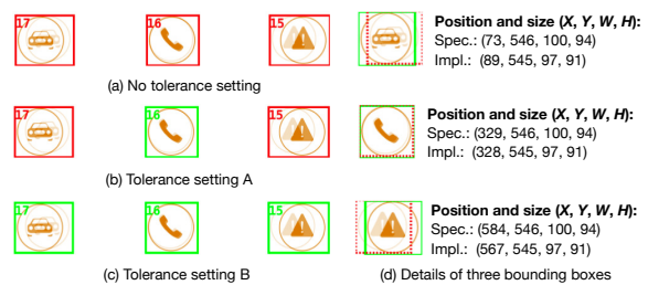
Figure 7. Flexible tolerance ( \Delta X, \Delta Y, \Delta W, \Delta H ) for examining bounding boxes. (a) No tolerance setting. (b) Tolerance setting A = (4, -1, 4, 4). (c) Tolerance setting b = (-1, -1, 4, 4). (d) Details of the bounding boxes.
